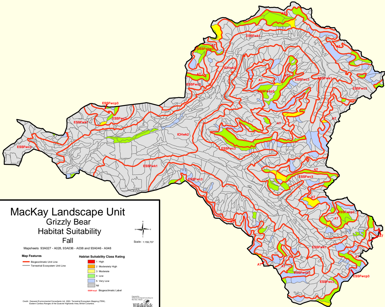
Figure 4. High value fall grizzly bear habitat within the Mackay Landscape Unit
