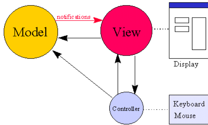
Model-View-Controller Scheme
