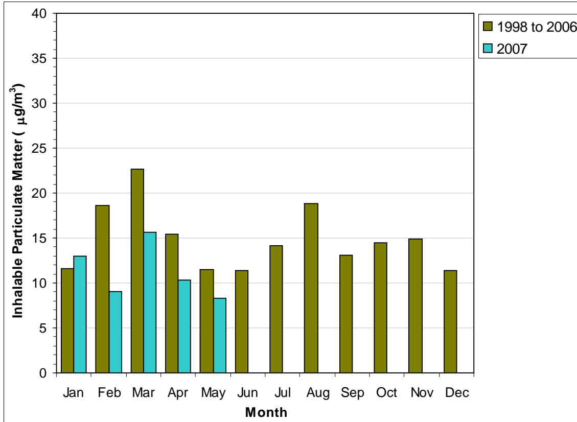
Figure 16: 2007 PM data compared with previous years.
