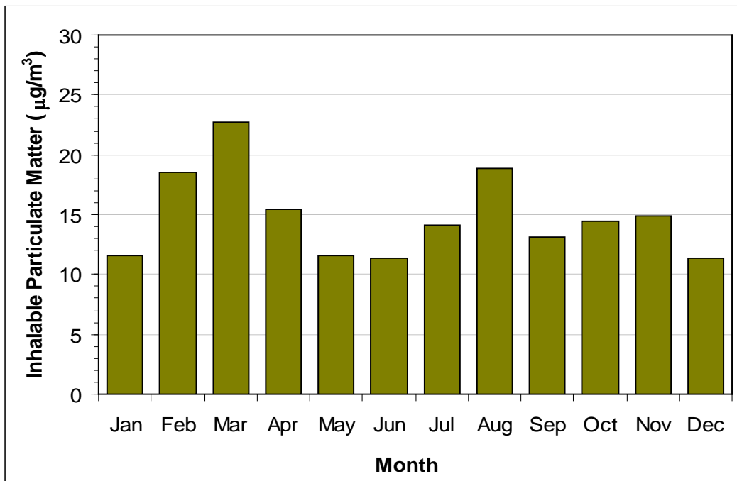
Figure 14: Monthly PM 10 concentrations. Radium’s daily mean PM 10 during the period 1998 to 2006 measured in each month are shown by the bars.
