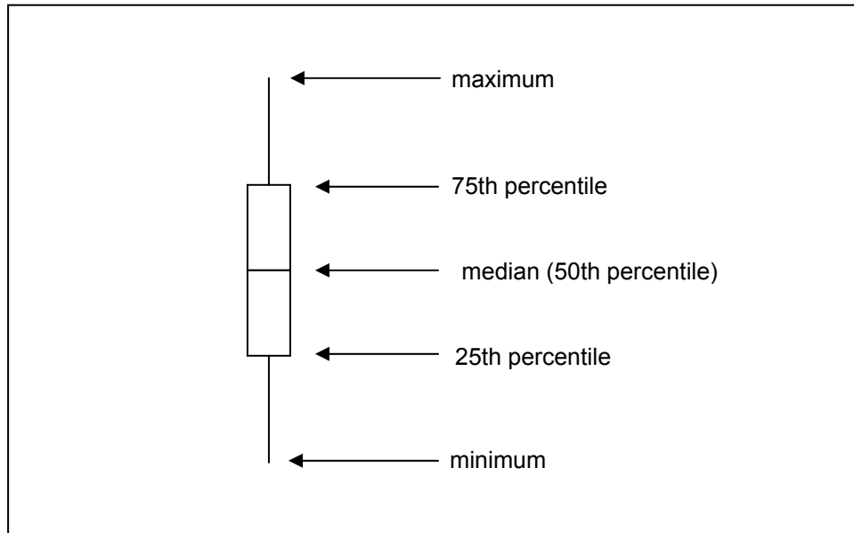
FIGURE C1. Boxplot
