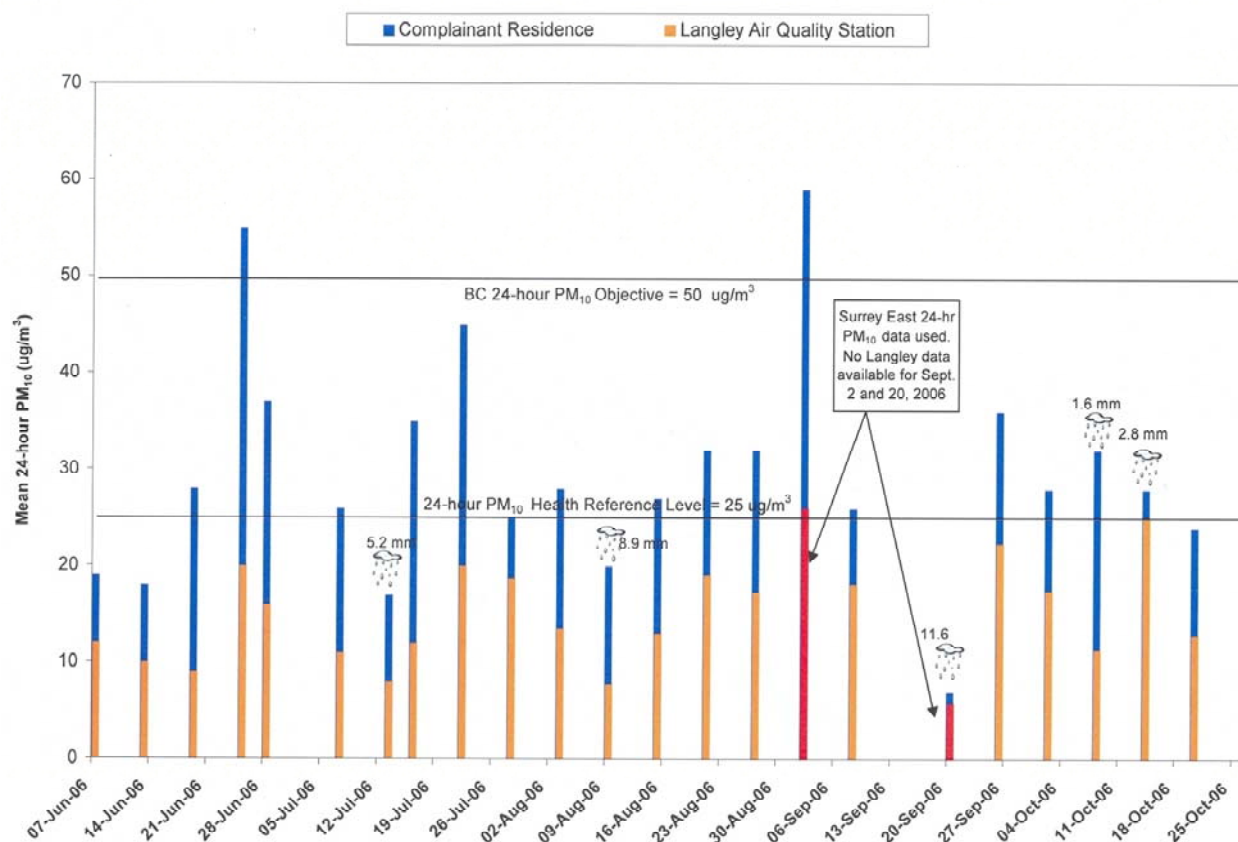
Figure 3 PM 10 sampling results for the complainant property and the background station. Note: Data from the Langley air quality station was gathered using a TEOM, whilst data from the complainant residence was collected using a Hi-Vol.
