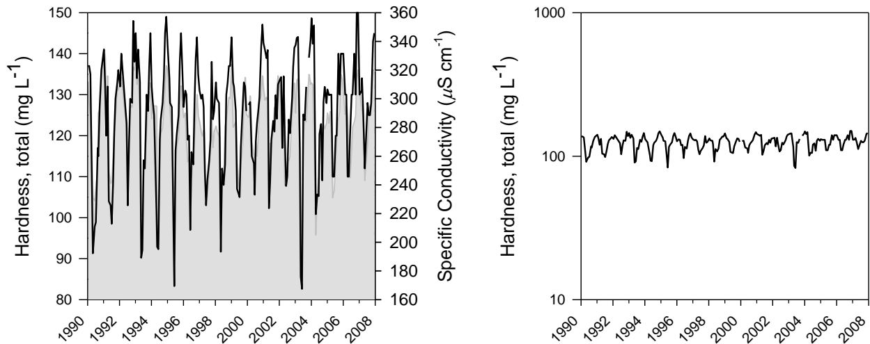
Figure 10: Total hardness concentrations in the Okanagan River from 1990 to 2008.
