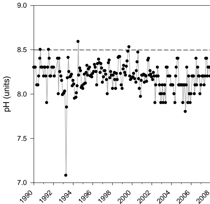
Figure 16: pH measurements in the Okanagan River from 1990 to 2008.
