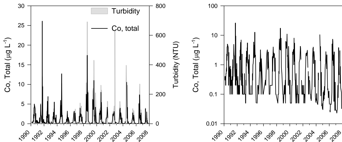
Figure 7: Total cobalt and turbidity (left) and total cobalt log-scale (right) concentrations from 1990 to 2008.
