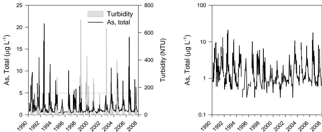
Figure 4: Total arsenic and turbidity (left) and total arsenic (log-scale) concentrations from 1990 to 2008. Dotted line represents the B.C. water quality criterion for aquatic life.
