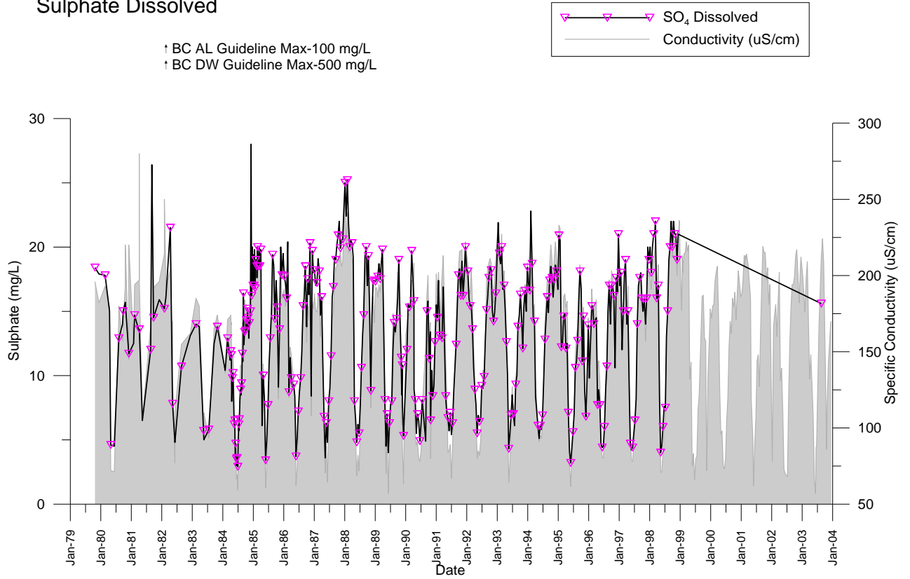
Figure 59 Similkameen River near U.S. Border Sulphate Dissolved
