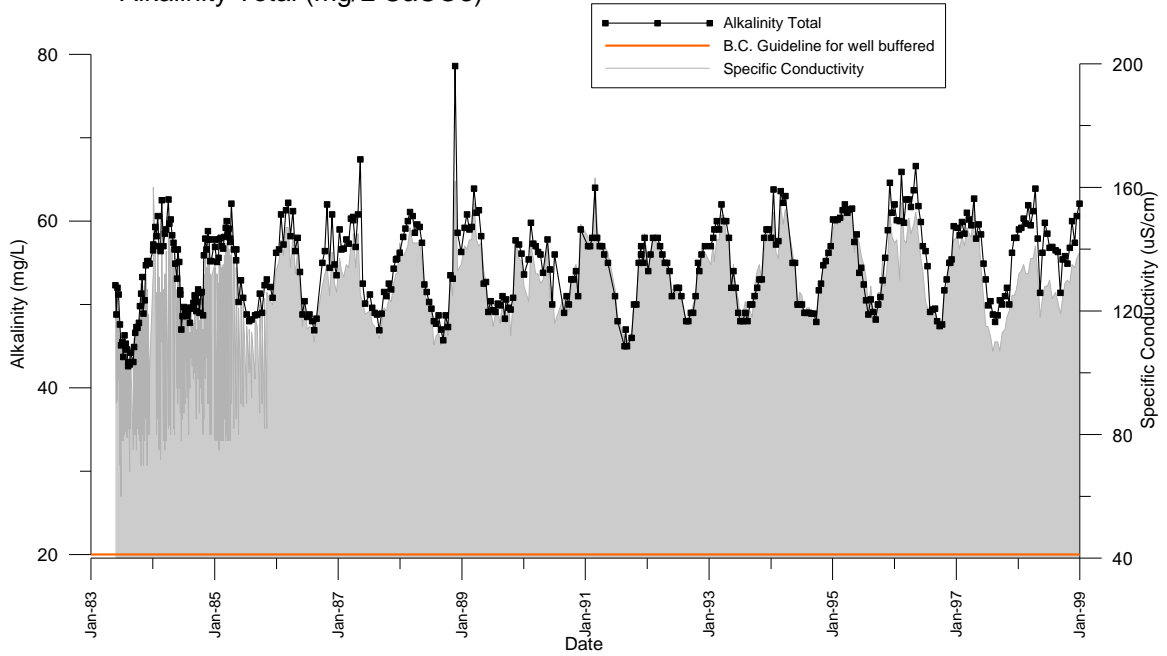
Figure 3 Columbia River at Birchbank Alkalinity Total (mg/L CaCO 3 )
