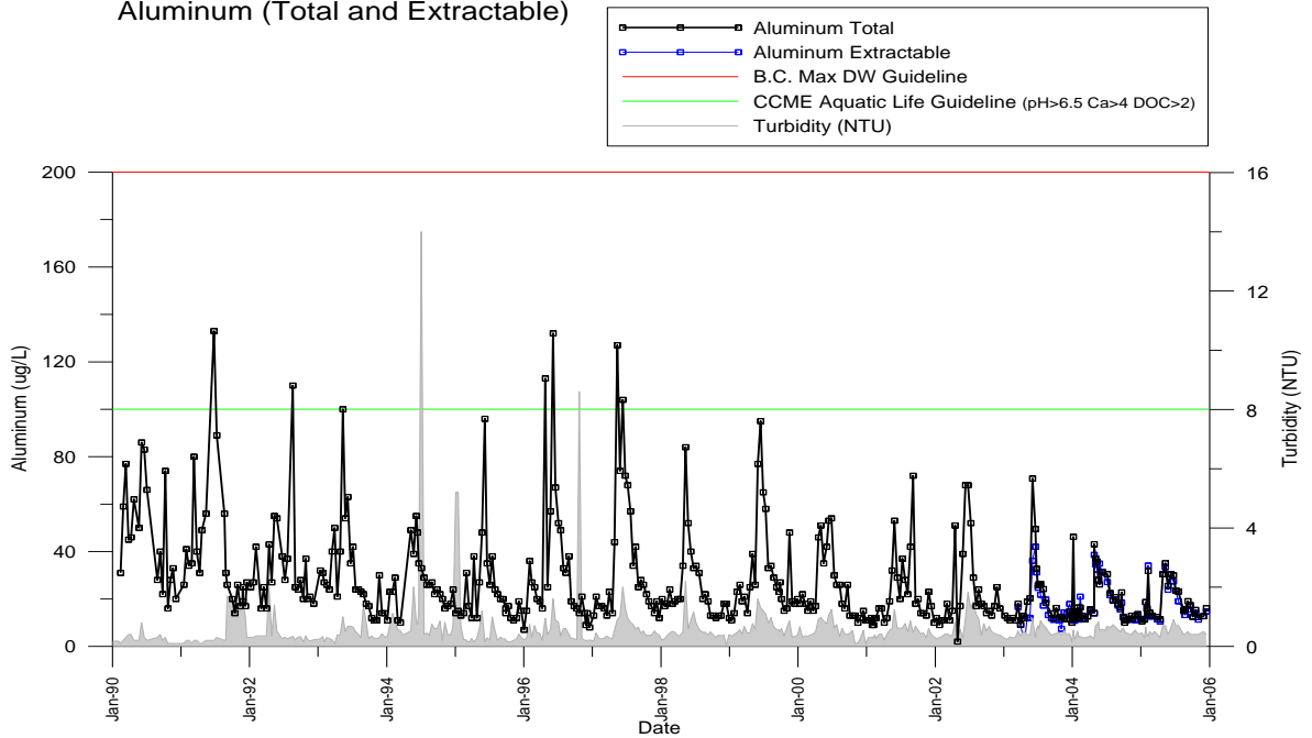
Figure 4 Columbia River at Birchbank Aluminum (Total and Extractable)
