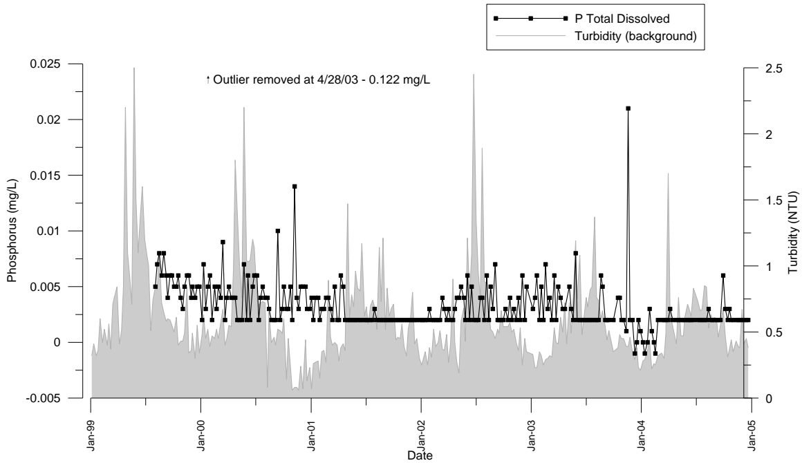
Figure 46 Columbia River at Waneta Phosphorus - Total Dissolved
