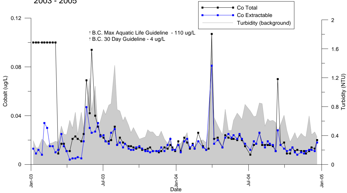
Figure 22 Columbia River at Waneta Colour - Apparent
