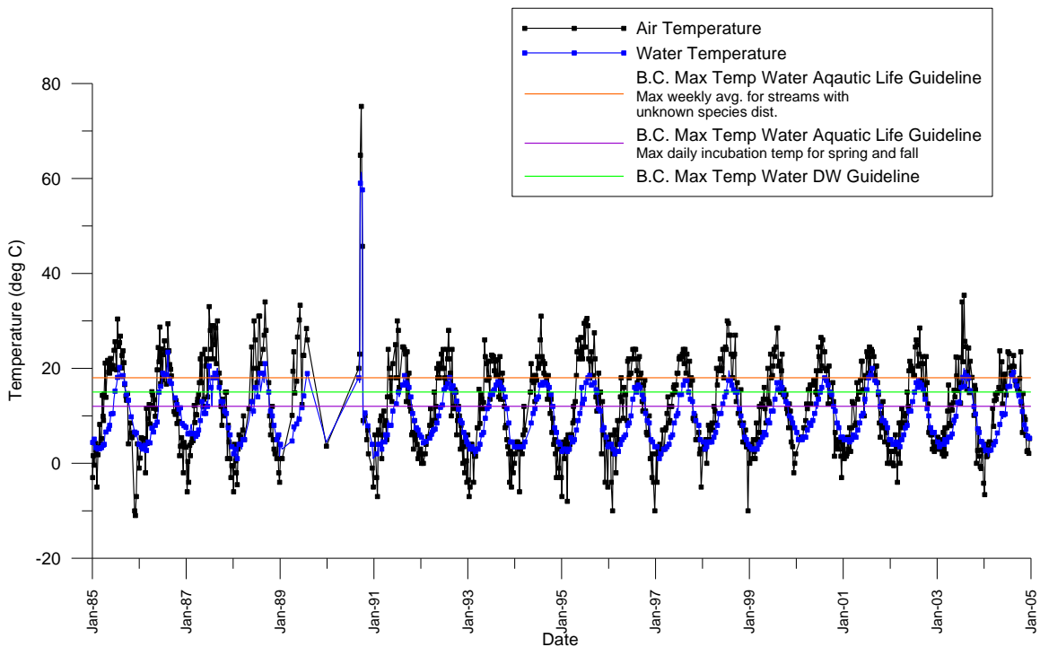
Figure 60 Columbia River at Waneta Temperature - Air and Water
