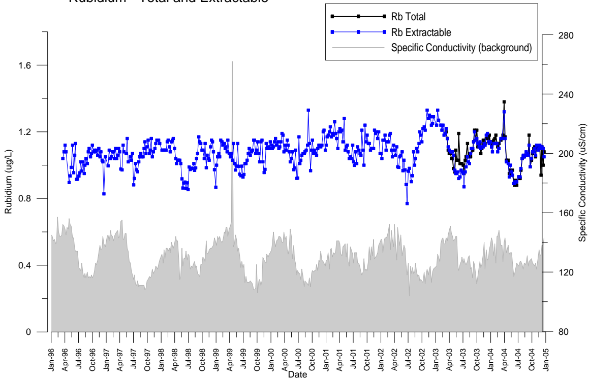
Figure 48 Columbia River at Waneta Rubidium - Total and Extractable
