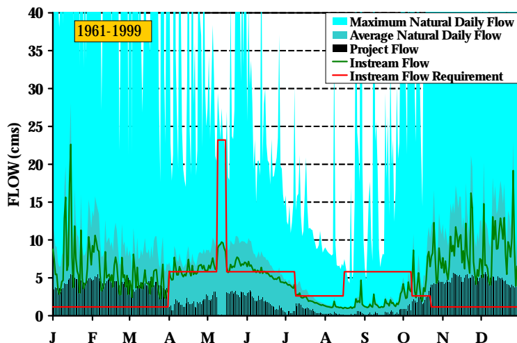
Figure 13. Simulated operations for a hypothetical run-of-river hydropower project for the Tsable River, Vancouver Island. The project has been operated to meet the instream flow requirements as calculated using the Ptolemy Method, for (A) 1992, a dry year, (B) 1997, a wet year, and (C) averaged from 1961 to 1999. Based on a MAD of 8.0 cms the instream flow requirements have been calculated and plotted as the solid red line. The blue shaded area shows the natural flows and the green solid line shows the instream flows released to meet the instream flow requirements. The black columns are flows diverted for the project.
