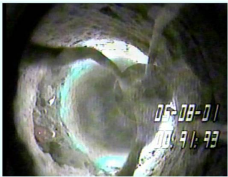
Biofilm and mineral deposits accumulate inside a water well over time
